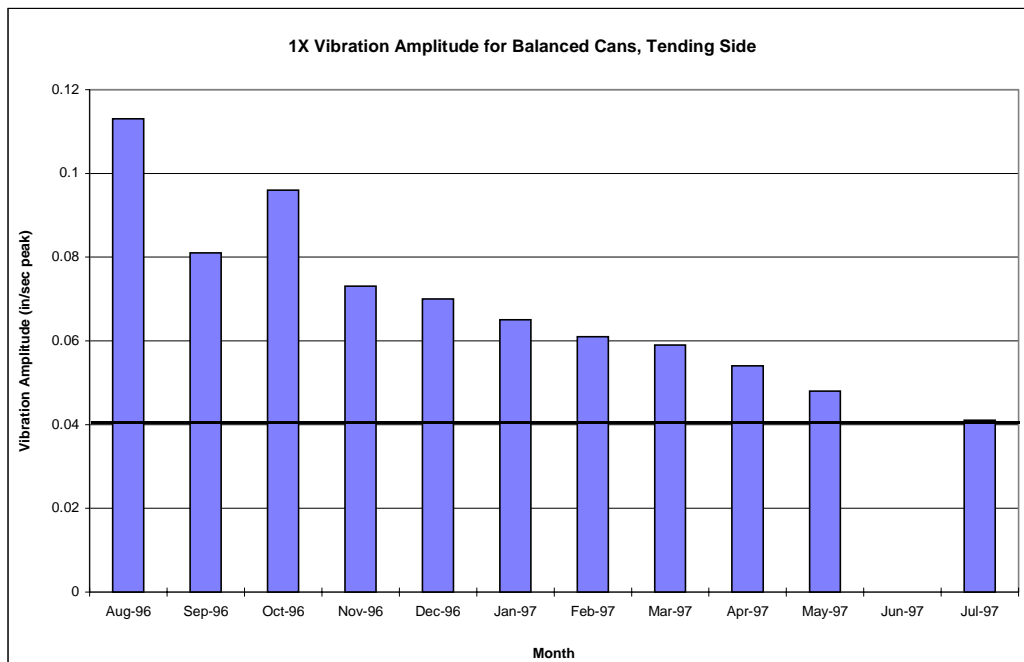
Fig 9 • Overall Project Results at Irving Paper Inc PM#2 (Note: Speed Increase 2800 to 3200 fpm)
