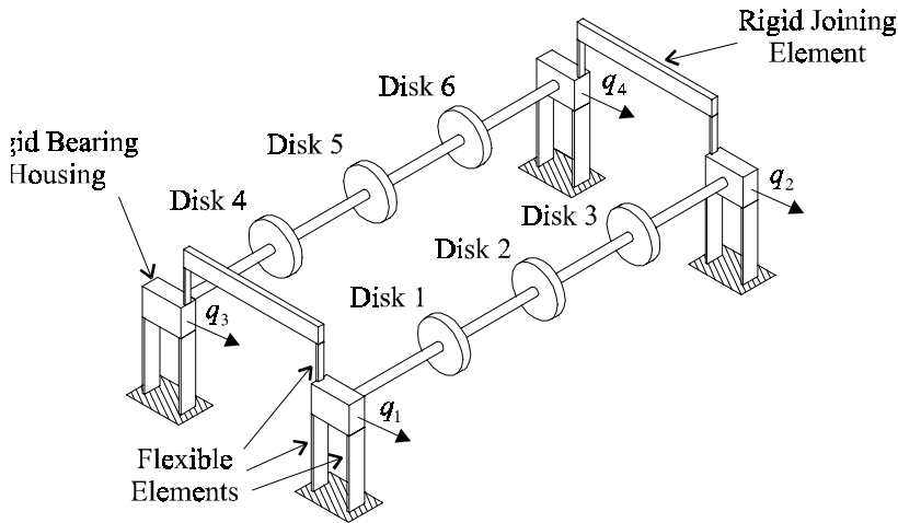
Fig 5 • Laboratory Test Model
