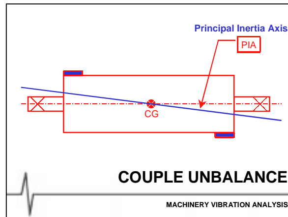
Fig 3 • Couple Unbalance
