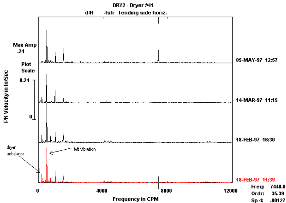
Fig 10 • Vibration Force due to Felt Roll Unbalance
