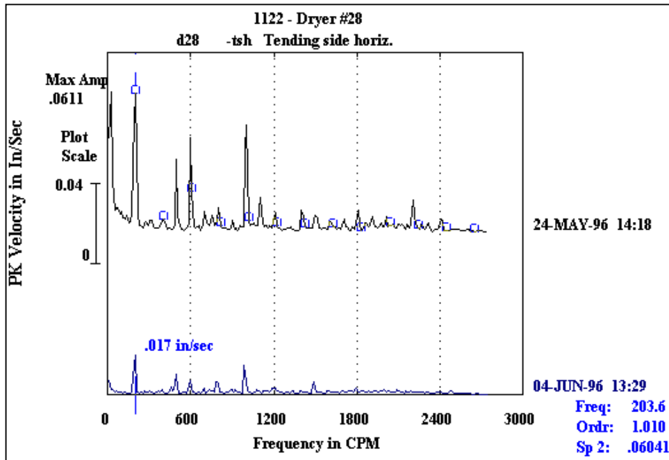
Fig 8 • 1 st Field Balance Attempt (Before and After Single Run Balance)
