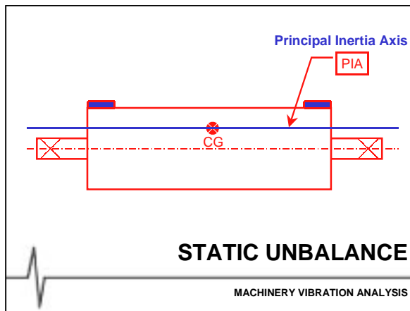
Fig 2 • Static Unbalance
